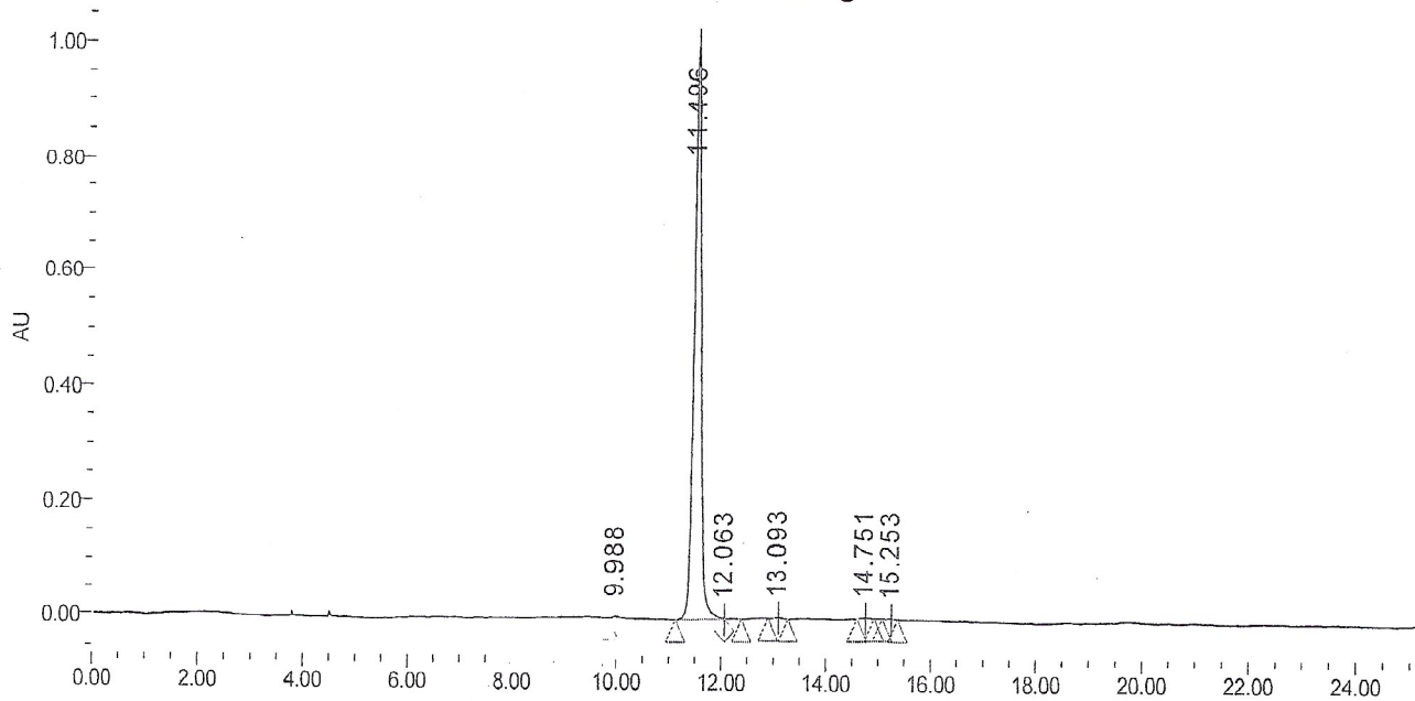
Auto-Scaled Chromatogram
